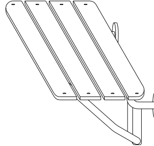
PHENOLIC SLAT SURFACE, W/O LEGS Mounts Right or Left hand
