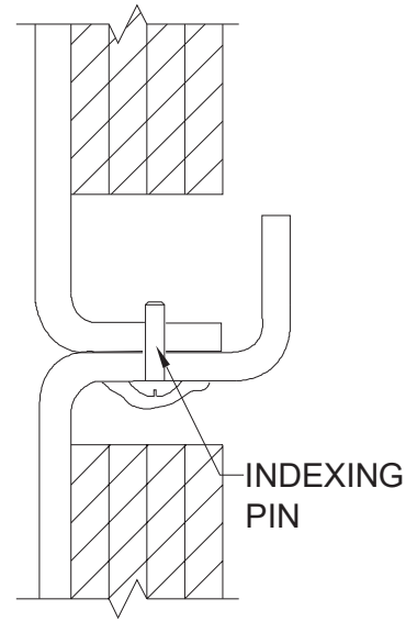
DETAIL B - SCALE N.T.S. WALL SECTION DETAIL
