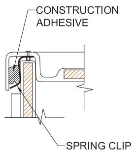
DETAIL B - SCALE: NTS WALL JOINT DETAIL
