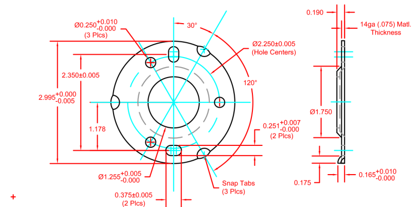
IQCR5-B-Flange Detail
