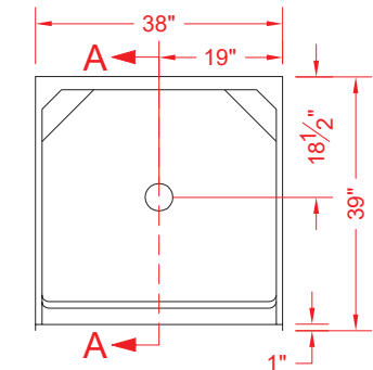
TOP VIEW - SCALE 3/8" = 1'-0"
