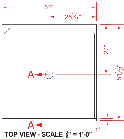
TOP VIEW - SCALE \frac{3}{8}'' = 1'-0''
