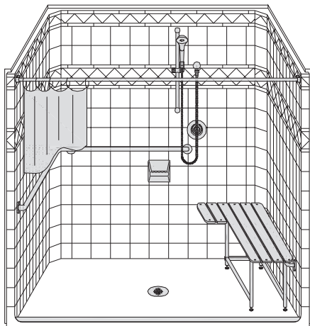
PERSPECTIVE VIEW - N.T.S. MODEL SHOWN HERE AS:
