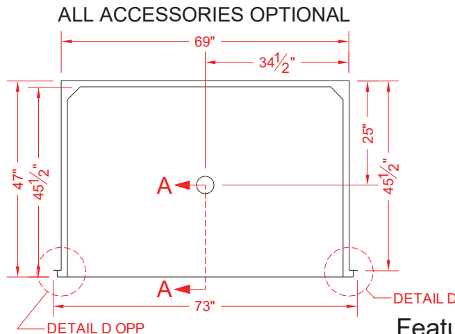
TOP VIEW - SCALE \frac{3}{8}'' = 1'-0''
