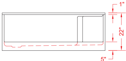
FRONT ELEVATION - SCALE: \frac{3}{8}'' = 1'-0'' * - SEE BACK FOR DETAIL SECTIONS
