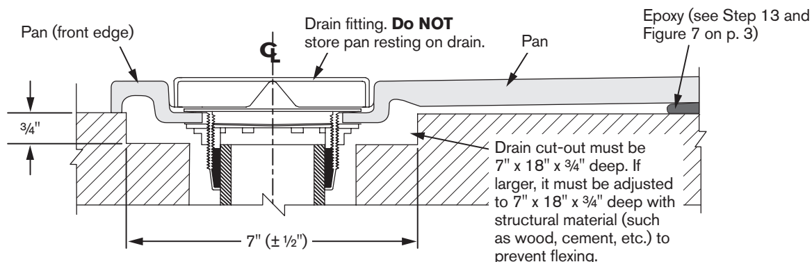
CROSS-SECTION OF SHOWER PAN (INSTALLED)
