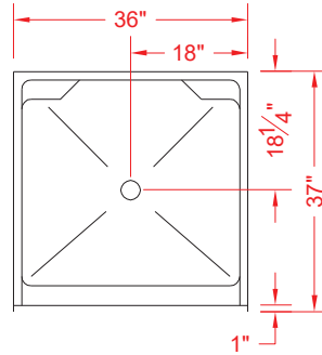
TOP VIEW - SCALE \frac{3}{8} " = 1'-0"
