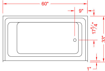
TOP VIEW - SCALE 3/8" = 1'-0"
