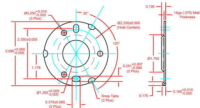
IQCR5-B-Flange Detail
