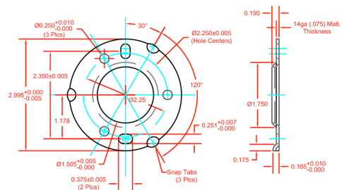
IHCR5-B-Flange Detail
